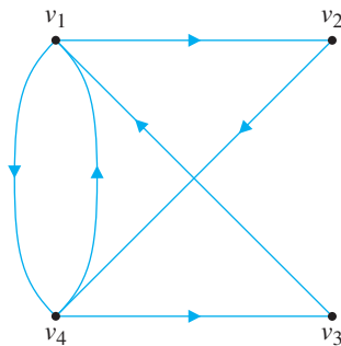
Figure 3.26 A digraph
