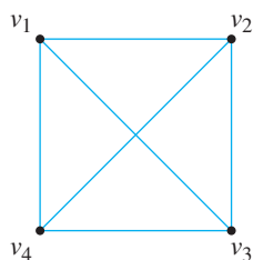
Figure 4.1 K_4
