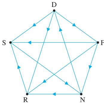
Figure 3.27 A tournament
