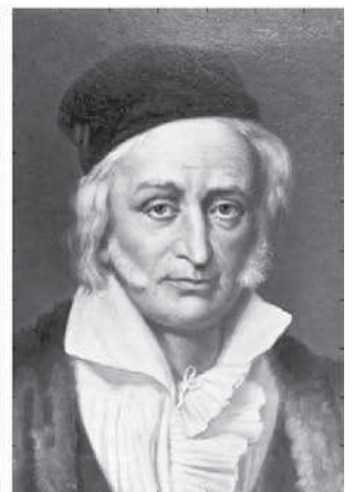
k = 256
