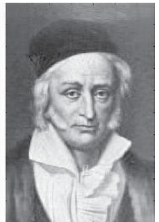
k = 32
