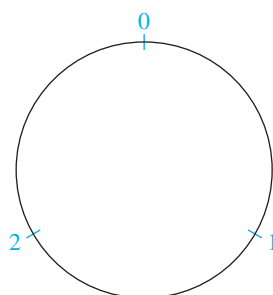
Figure 1.20 Arithmetic modulo 3
